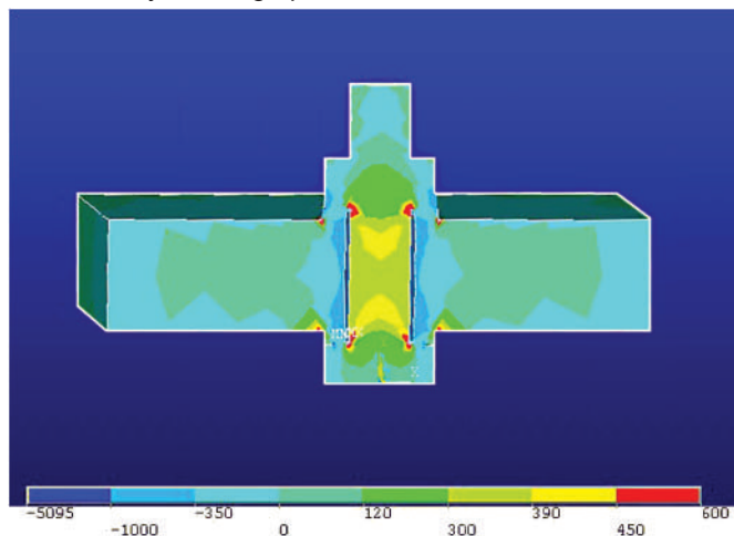
Stress increase in typical short bolt connections as a result of thermal stretch. The stress levels do not include prestress from bolt installation torque.
